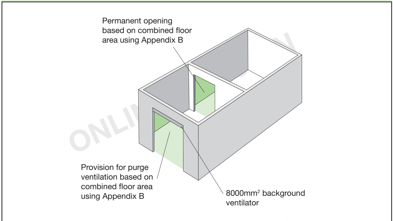
Diagram 2 Two habitable rooms treated as a single room for ventilation purposes
